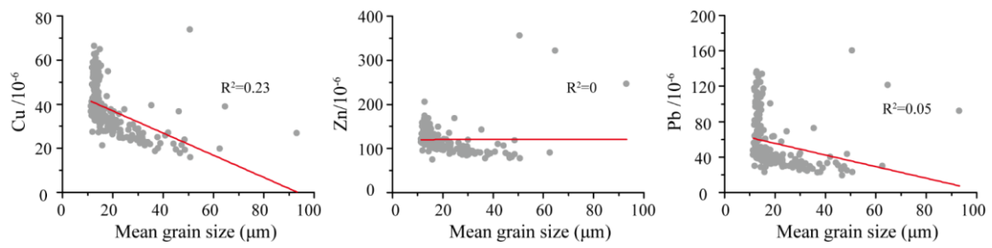
Fig. S1. The correlations between the mean grain size and the concentrations of Cu, Zn, and Pb in core HOBAB4-S2.
